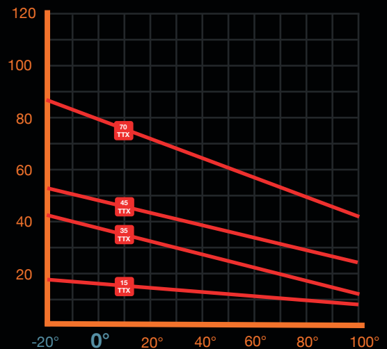
Temperature (°C) / Loading (W/m) diagram
